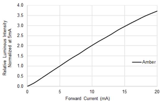
Fig.4 Relative Luminous Intensity vs. Forward Current
